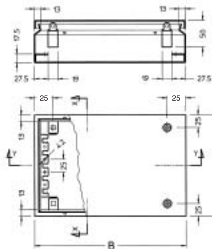
section Y-Y
